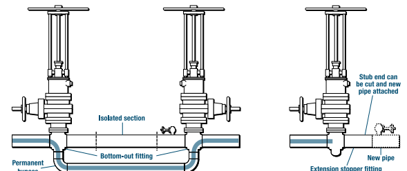
By-pass/double stop-off using bottom-out or side-out fittings - up to 500 psig
