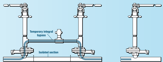
By-pass/double stop-off - up to 100 psig
