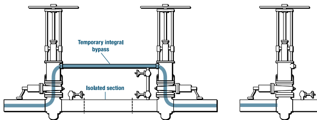
By-pass/double stop-off - up to 500 psig
